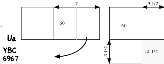
Figure 10. YBC 6967, after Neugebauer and Sachs [20, pl. 17].
