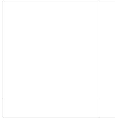
Figure 7. Diagram from which follows “proto- Elements II.7,” \square(R-r) = \square(R) - 2\square(r) + \square(r) .
